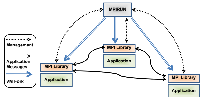
Figure 3: SnowFlock MPI Architecture. The SnowFlock MPI implementation just has a single MPI management process on the master VM, which runs only as long as the application processes and handles all their management traffic.
