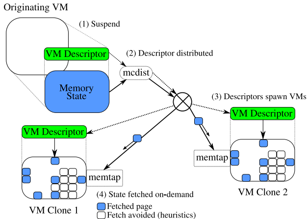
Figure 1: SnowFlock VM Replication Architecture. Condensed VM descriptors are distributed to cluster hosts to spawn VM replicas. Memtap populates the VM replica state on demand, using multicast distribution. Avoidance heuristics reduce the number of necessary fetches.
