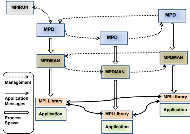
Figure 2: Standard MPI Architecture. The standard MPI architecture involves a persistent one-way ring of management processes (mpd), and another one-way ring that manages each application run (mpdman). Control messages travel through the rings, while workers exchange application messages point-to-point.
